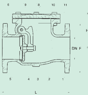
CLAPET A BRIDES DOUBLE FLANGED CHECK VALVE
