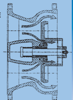
CLAPET LINEAIRE SPRING CHECK VALVE
