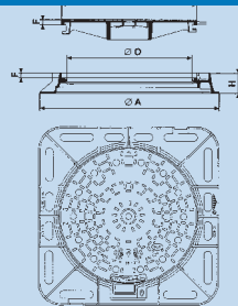
PLAQUES FONTE REGARD MANHOLE COVER AND GRATING
