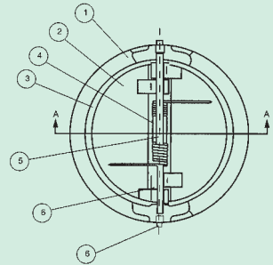
CLAPET SANDWICH CHECK VALVE WAFER TYPE
