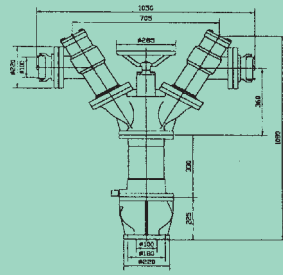
BORNE IRRIGATION IRRIGATION HYDRANT
