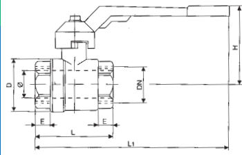
ROBINET BOISSEAU SPHERIQUE DOUBLE FEMALE BALL VALVE
