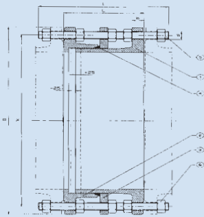
RACCORDS GALVANISES GALVANIZED FITTINGS
