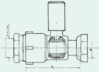
ROBINET INVIOLEBLE INVIOLEBLE WATER METER COCK
