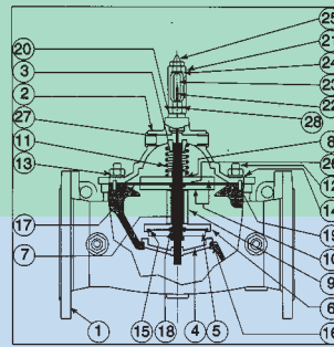
STABILISATEUR AMONT ET AVAL UPSTREAM AND DOWNSTREAM SUSTAINING VALVE
