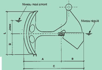
VANNE VANIS CONSTANT DOWNSTREAM LEVEL GATE
