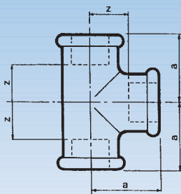
RACCORDS GALVANISES GALVANIZED FITTINGS
