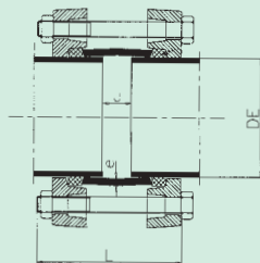
JOINTS GIBAUT STRAIGHT COUPLING
