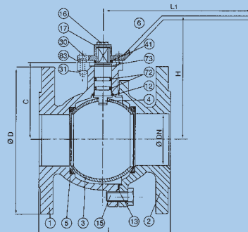
VANNE BOISSEAU SPHERIQUE A BRIDES DOUBLE FLANGED BALL VALVE
