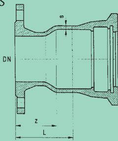
JOINT DE DEMONTAGE AUTOBUTE DISMANTLING JOINT
