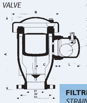
VENTOUSE 3 FONCTIONS KINETIC AIR RELEASE VALVE
