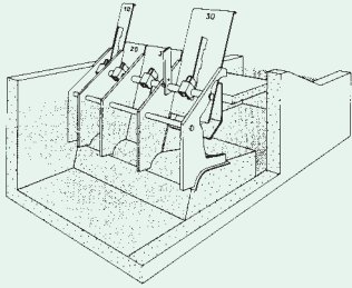
VANNE CALIFORNIENNE OVERFLOW RISER VALVE
