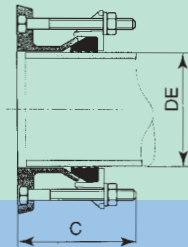
ADAPTATEURS A BRIDE LARGE TOLERANCE WIDE TOLERANCE ADAPTOR
