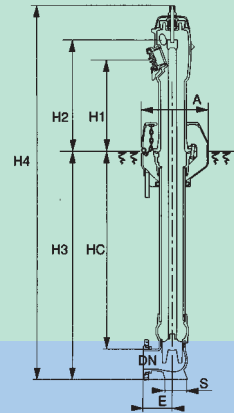
POTEAU INCENDIE PILLAR FIRE HYDRANT
