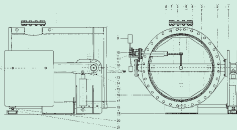
STABILISATEUR AMONT ET AVAL UPSTREAM AND DOWNSTREAM SUSTAINING VALVE
