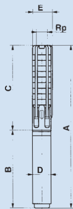
POMPE IMMERGEE SUBMERSIBLE PUMP
