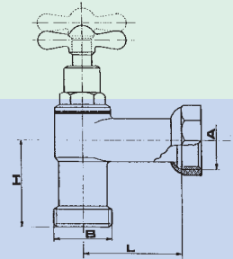
ROBINET EQUERRE 90° KEY TYPE METER COCK
