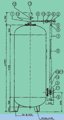
BALLON ANTI BELIER ANTI-HAMMER TANK
