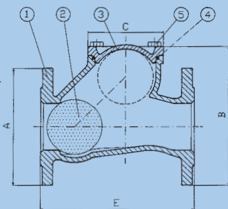
CLAPET A BOULE DOUBLE FLANGED BALL CHECK VALVE
