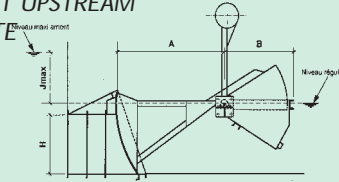
BORNE IRRIGATION IRRIGATION HYDRANT
