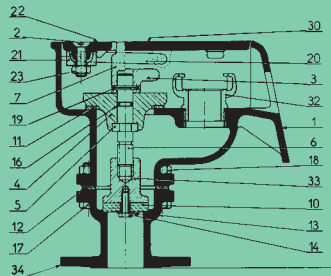
BOUCHE INCENDIE UNDERGROUND FIRE HYDRANT
