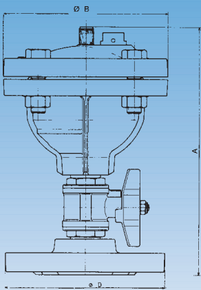
VENTOUSE 1 FONCTION SINGLE ACTION AIR RELEASE VALVE
