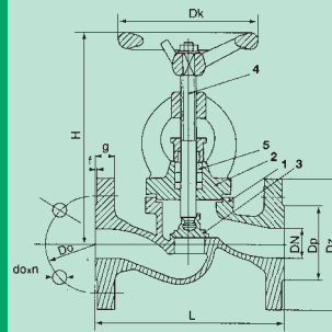
ROBINET A SOUPAPE CAST IRON GLOBE VALVE
